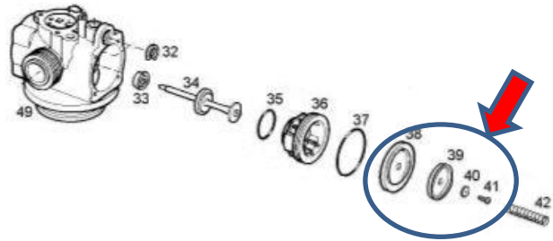
Image 2: Current version of retainer with additional washer
